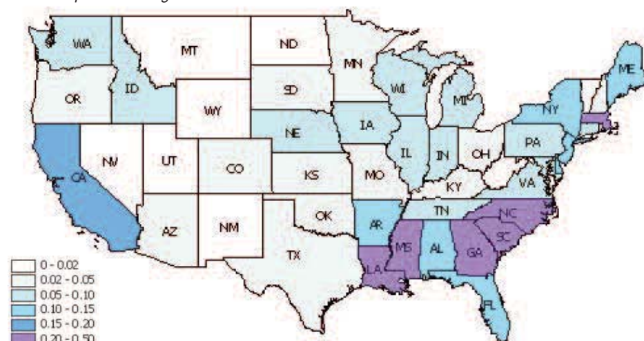
Figure 5. Proportion of the total 1997 US farmland area where the use of pesticides created a situation where bird deaths were expected. Numbers are expressed as probabilities with the maximum possible being 1.
